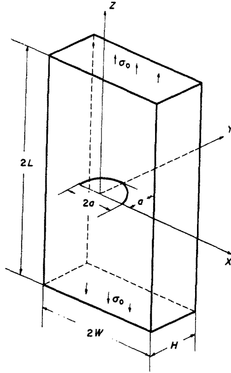
Fig. 6. Semi-circular surface crack in block under uniform tension.
