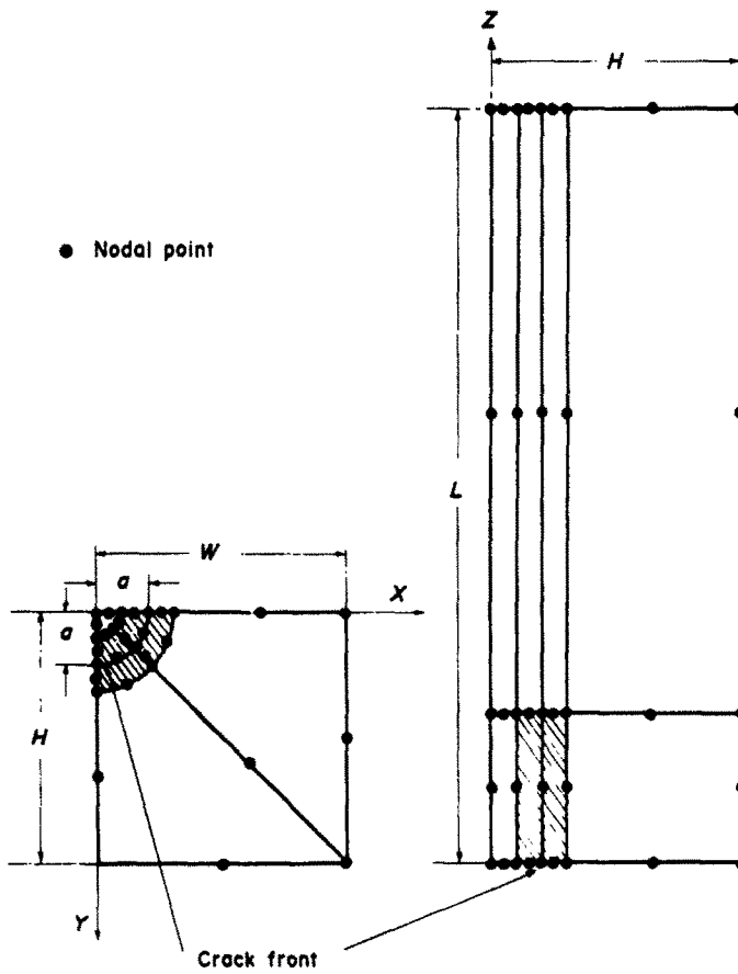
Fig. 7. Mesh subdivision for one quarter of the block with a crack.
